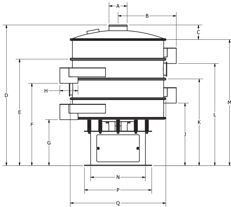
24" & 30" Triple Deck With Cover
